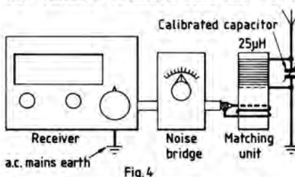
Fig. 4: Shows connection of receiver to noise-bridge and on to the matching unit. Note the use of r.f. and a.c. mains earthing
