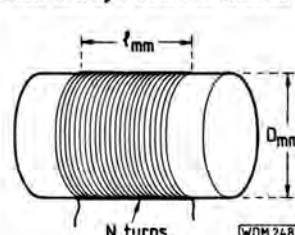
Fig. 5: Coil former showing dimensions used in calculating its inductance, dimensions in millimetres
