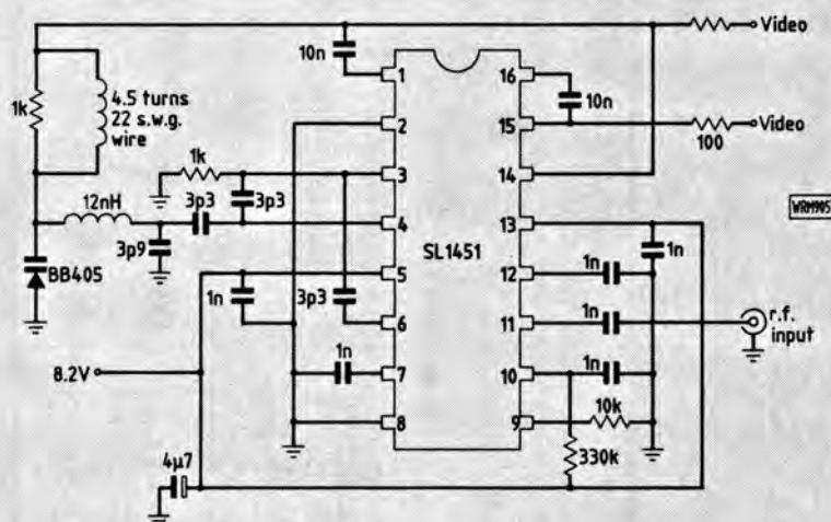
Fig. 3: A typical practical circuit using the SL1451 EXP as an f.m. demodulator
