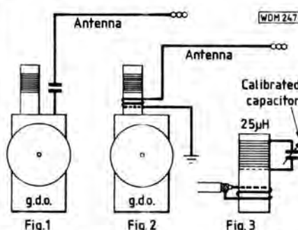
Fig. 1: Capacitive coupling of g.d.o. to antenna
